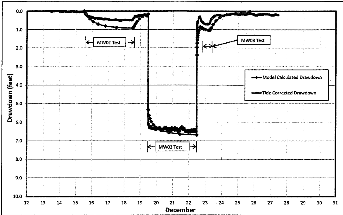
Figure 11 - Calculated versus Observed Drawdown, Phase 1 Testing, MCWP-MW01
