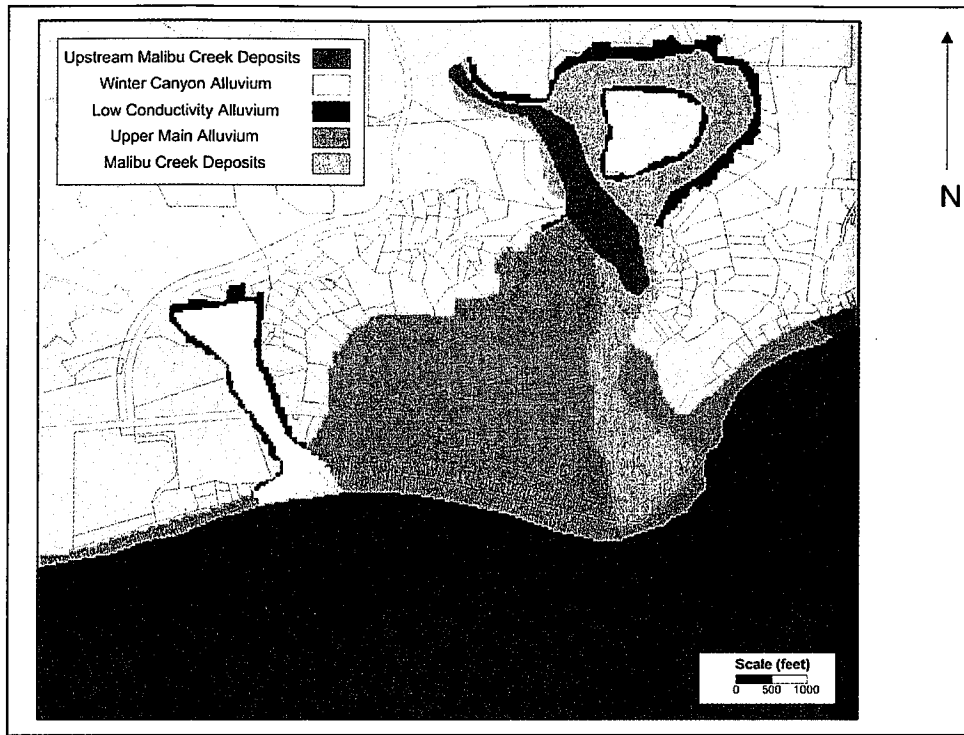
Figure 15 - Hydraulic Conductivity Zones in Model Layer 1
