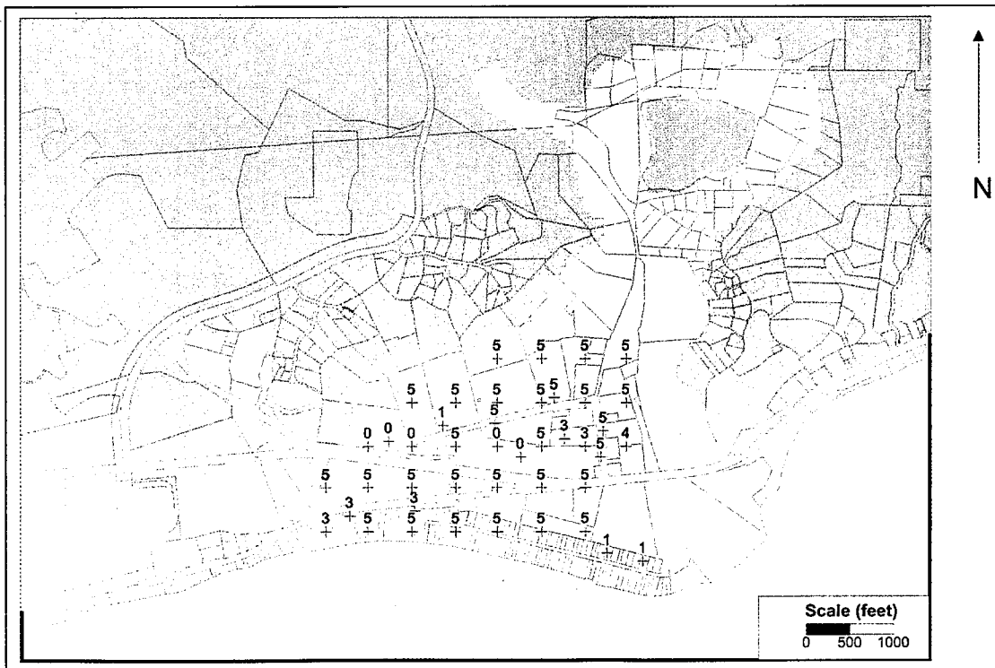
Figure 20 - Acceptable Depth-to-Water at Each Constraint Location
