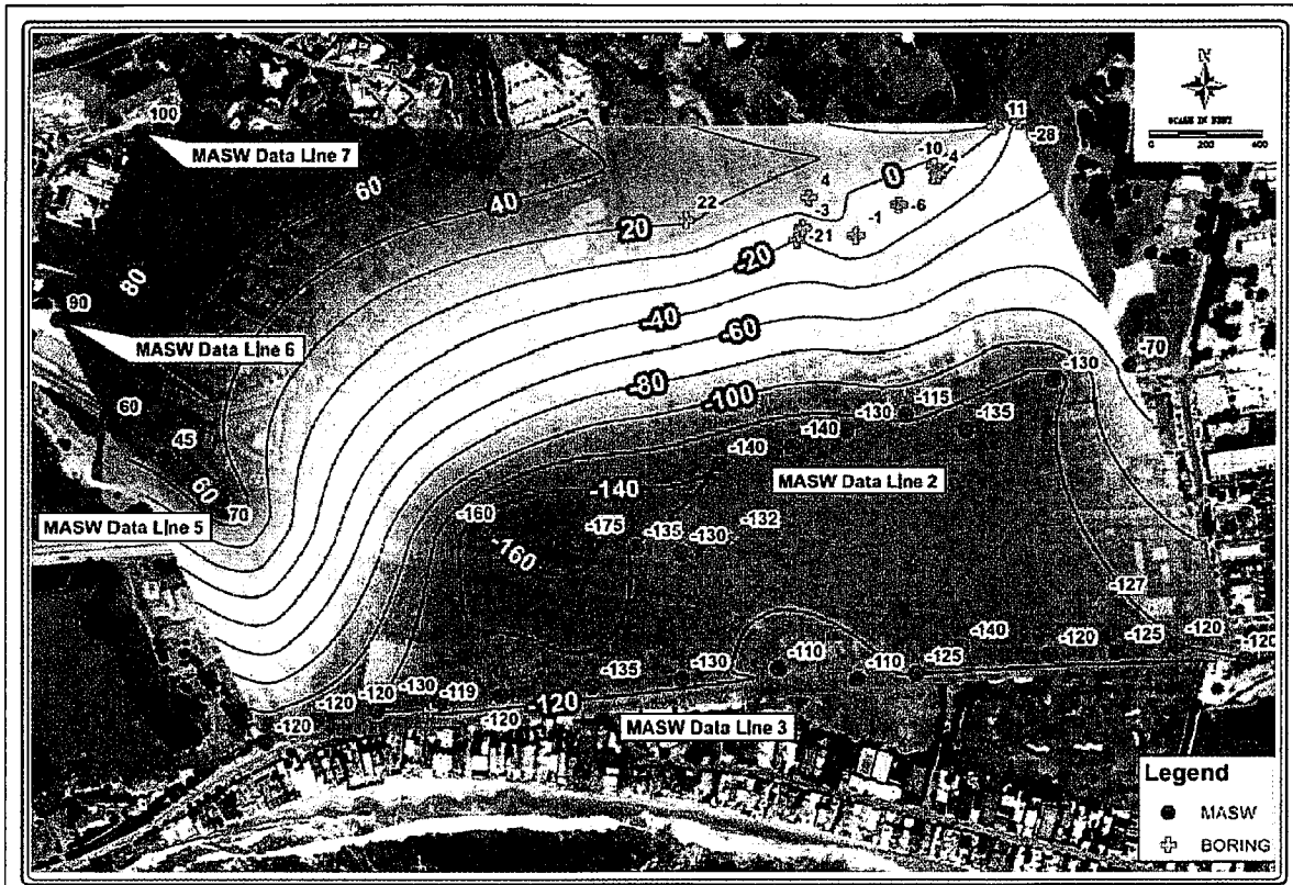
Figure 3 - On-shore Bedrock Mapping of Civic Center Area
