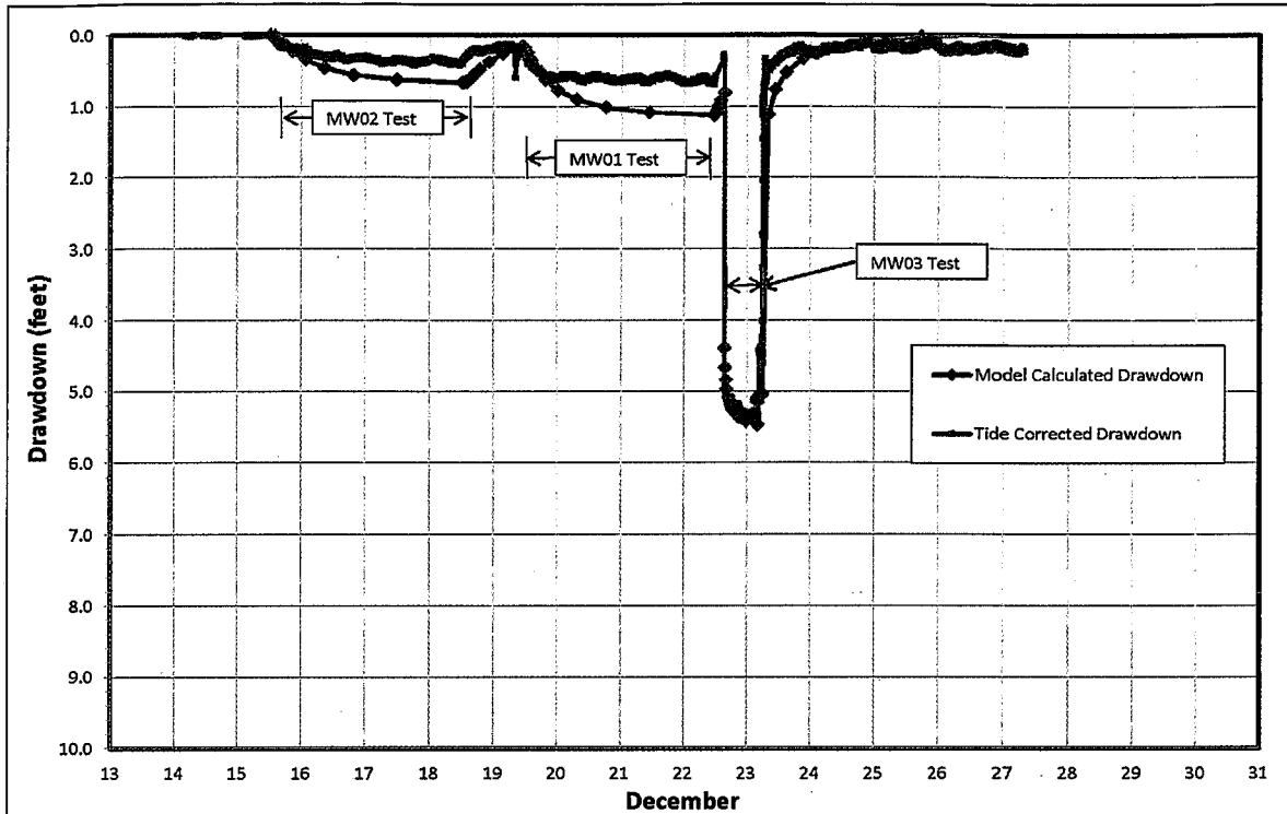
Figure 13 - Calculated versus Observed Drawdown, Phase 1 Testing, MCWP-MW03
