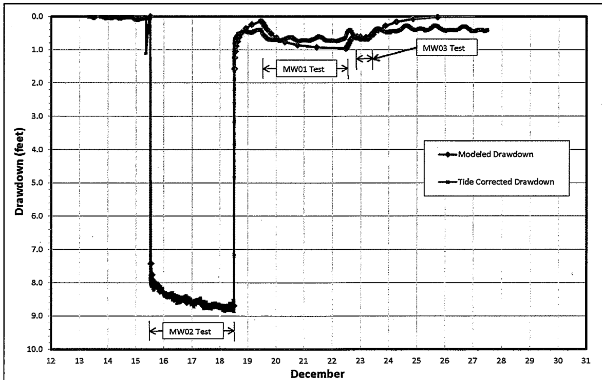
Figure 12 - Calculated versus Observed Drawdown, Phase 1 Testing, MCWP-MW02
